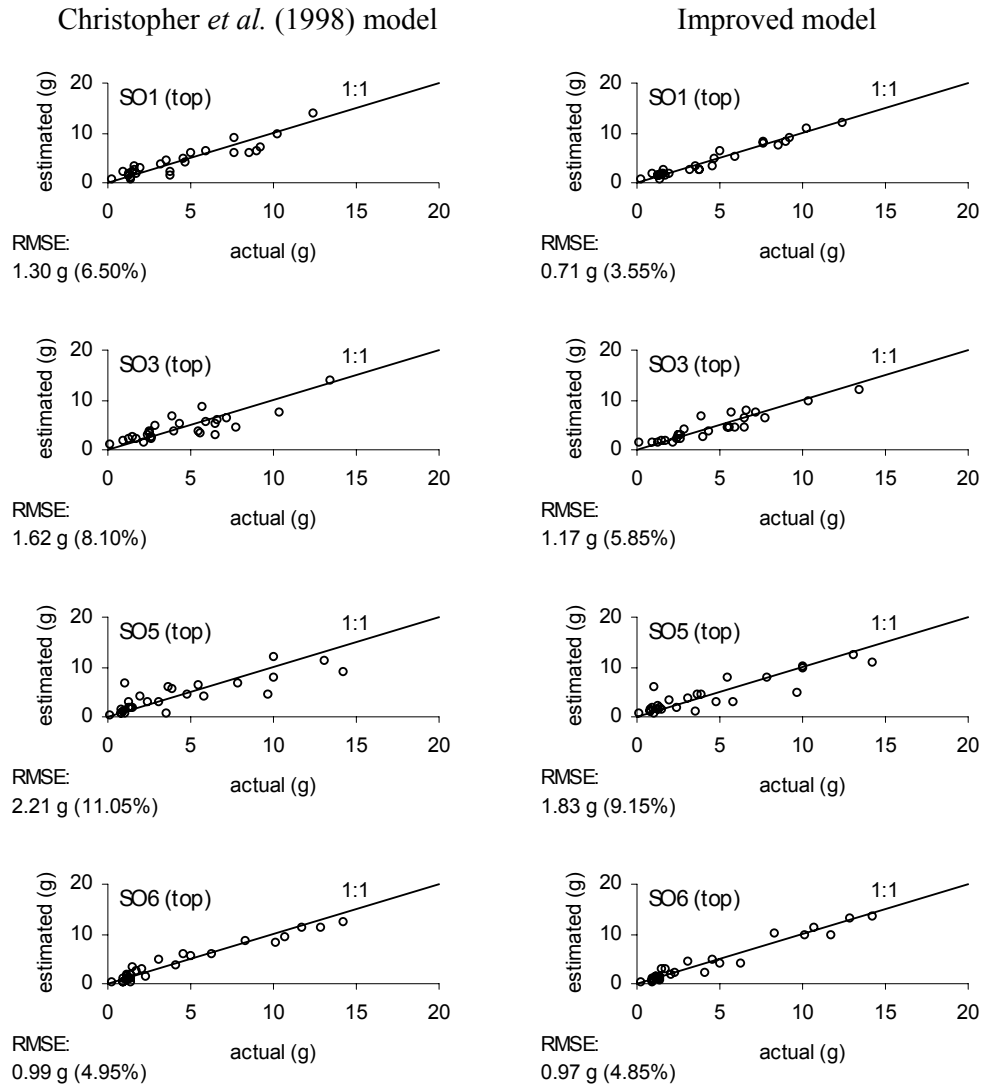
FIGURE 2. Comparisons Between the Estimated and Actual Weight of Retained Aggregates w_{i,\dots,j} for Selected Soil Types (0-150 mm soil depth). Graphs in the Left and right columns are the performance of the Christopher et al. (1998) model and the improved model, respectively.
