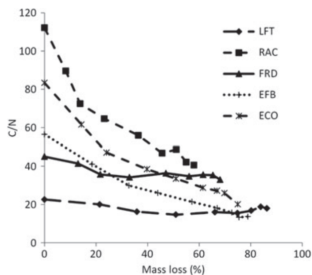
Figure 7 The relationship between C/N ratio and mass loss for various oil palm residues during decomposition. LFT, RAC, FRD, EFB and ECO denote leaflets, rachis, pruned palm fronds, empty fruit bunches and Eco-mat, respectively.
